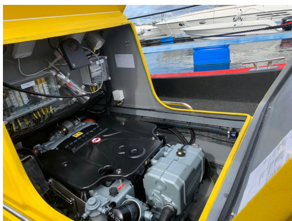
NANNI T8V.370 engine - Swedish rescue boat
